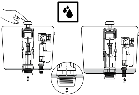
OPERATION MODE DUAL FLUSH
