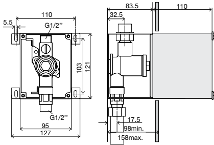
Urinal concealed pre-installation
